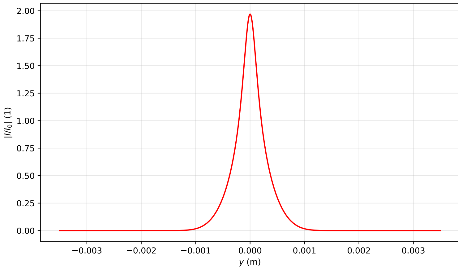
Intensity profile I(x = 0, y, z = 0.239)/I_0 , P_{in}=8.0P_{cr} , artificial time
